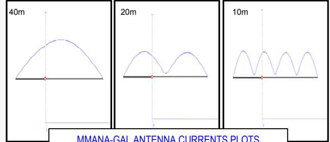
MMANA-GAL ANTENNA CURRENTS PLOTS
